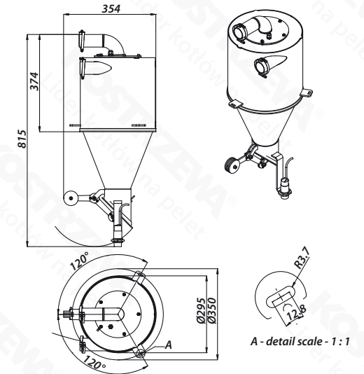
suction tank
