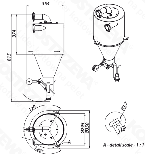
suction tank
